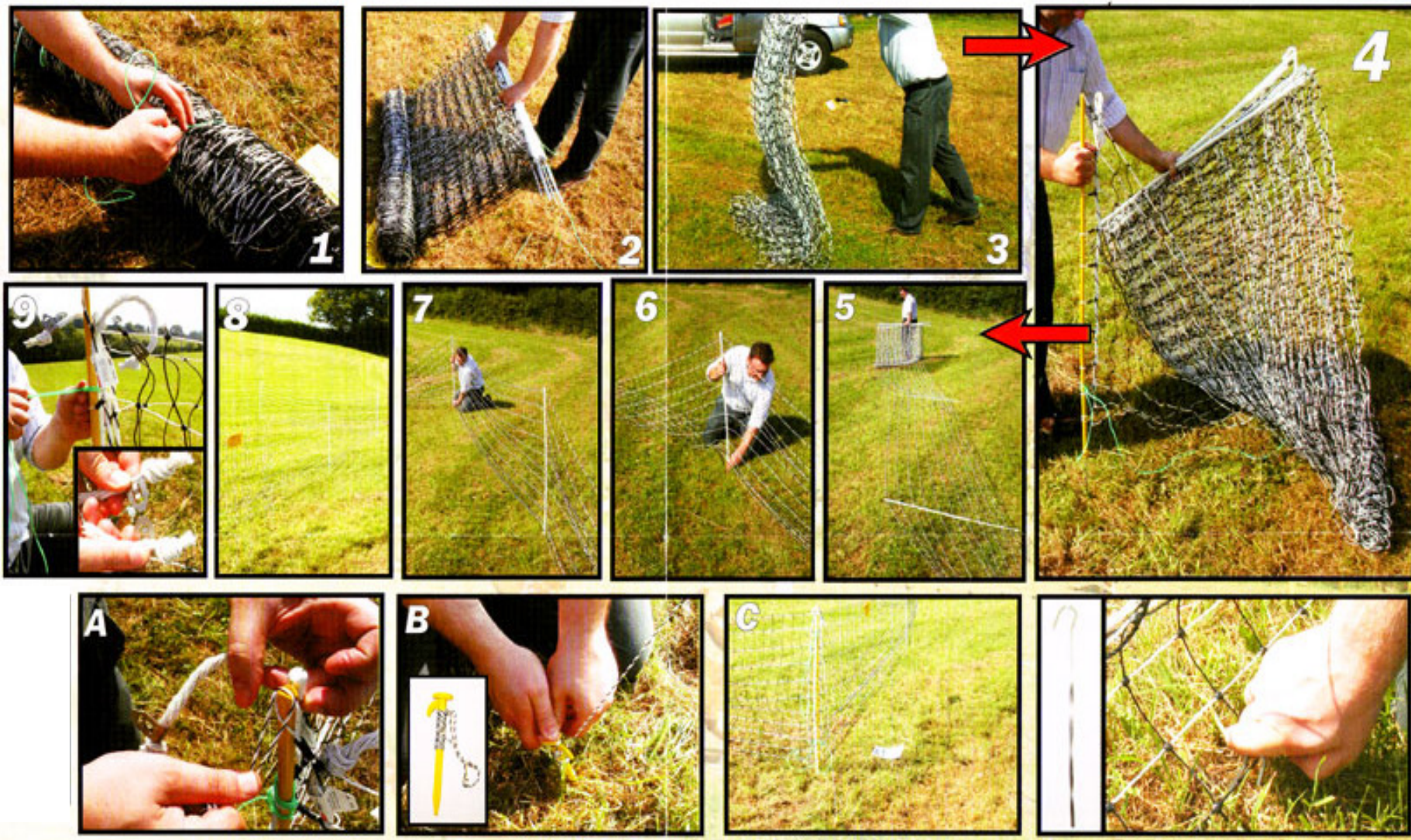
Erecting Electric Netting: Nos 1 - 9 Putting the Net up; Nos 9 - 1 Taking the Net down. Figs A & B - fixing the Guy Ropes to corner posts for tensioning. Fig C -Warning Sign. Fig - D Anchoring Pegs
